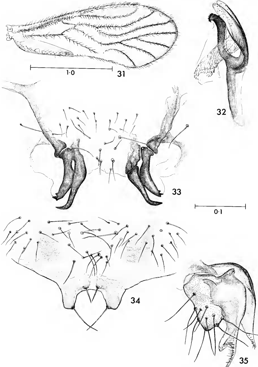
FIGS 31-35. — Lobocaeilius nigroides , ♂ holotype : 31, fore wing; 32, phallosome (side view); 33, hypandrium. ♀ allotype : 34, subgenital plate; 35, gonapophyses. (Figs 32-35 to common scale.)
